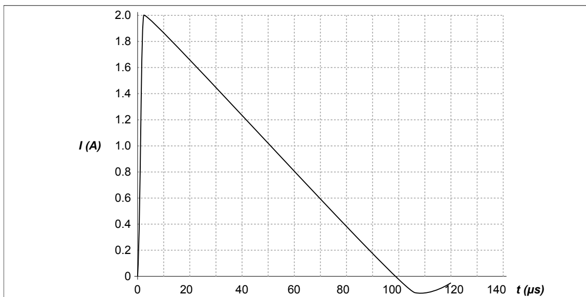
Fig. 20: Surge waveform
