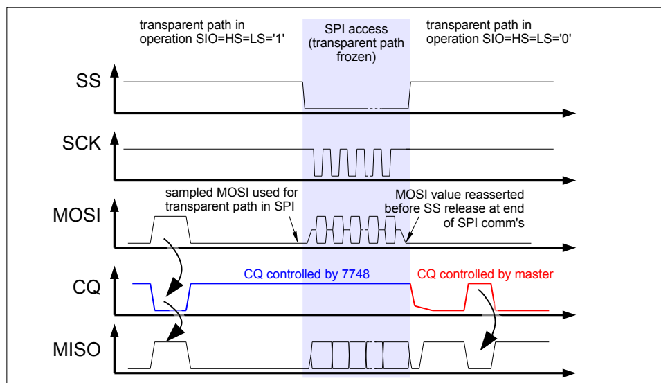
Fig. 10: Illustration of operation in transparent mode
