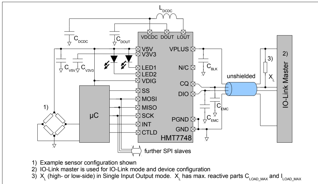
Fig. 4 DCDC in use, CQ/DIO driven independently, VDIG=V5V
