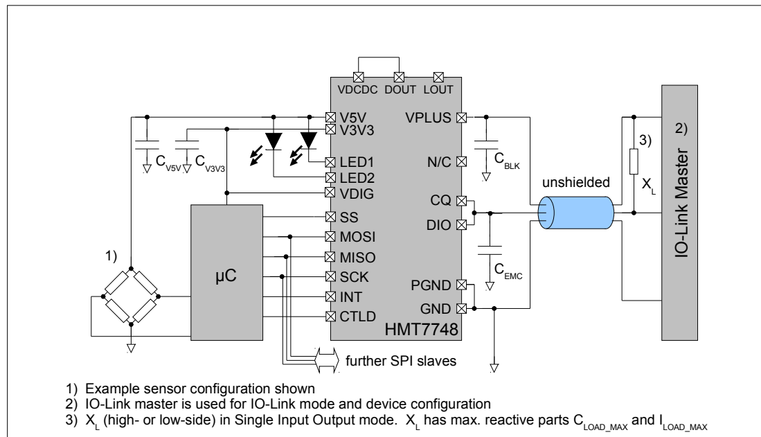
Fig. 5 DCDC bypassed, CQ/DIO driven in JOIN mode, VDIG=V3V3
