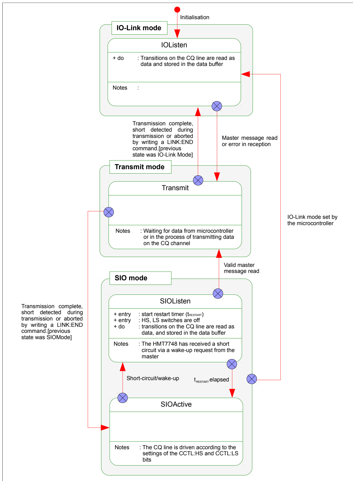
Fig. 8: IO-Link UART peripheral state machine
