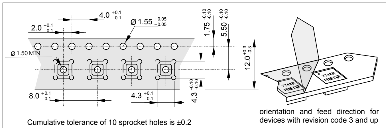
Fig. 22 Package, footprint and tape drawings for QFN
