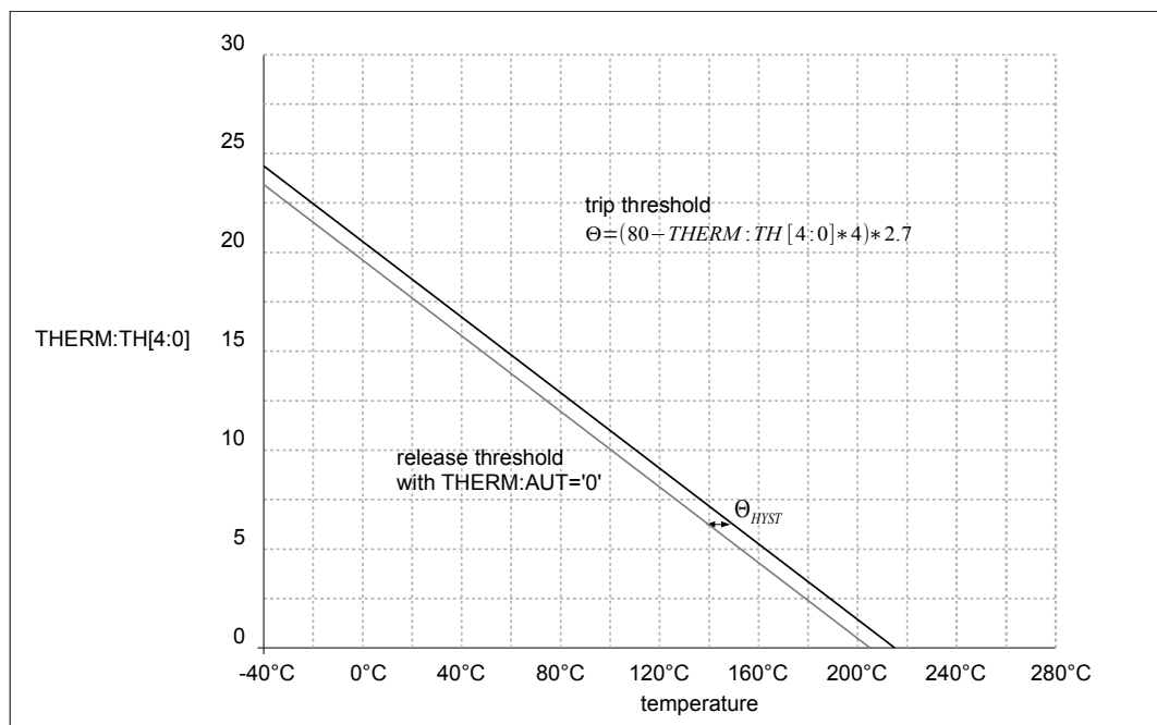
Fig. 12 HMT7748 thermal shutdown configuration
