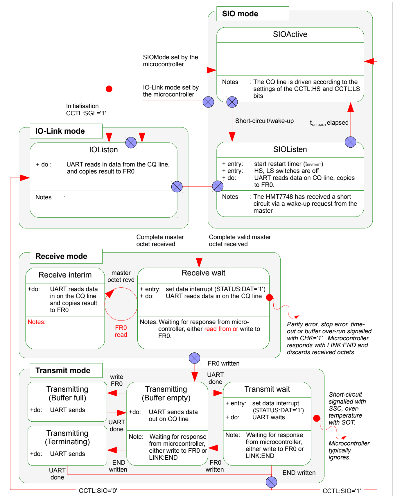
Fig. 9: Single octet UART mode state diagram
