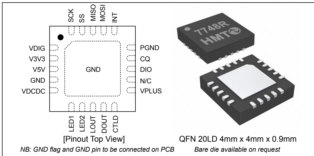
Fig. 2: Package and pinout - QFN
