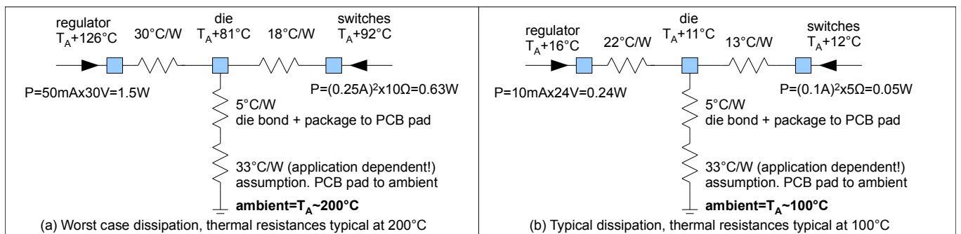
Fig. 18: Example thermal power dissipation estimation
