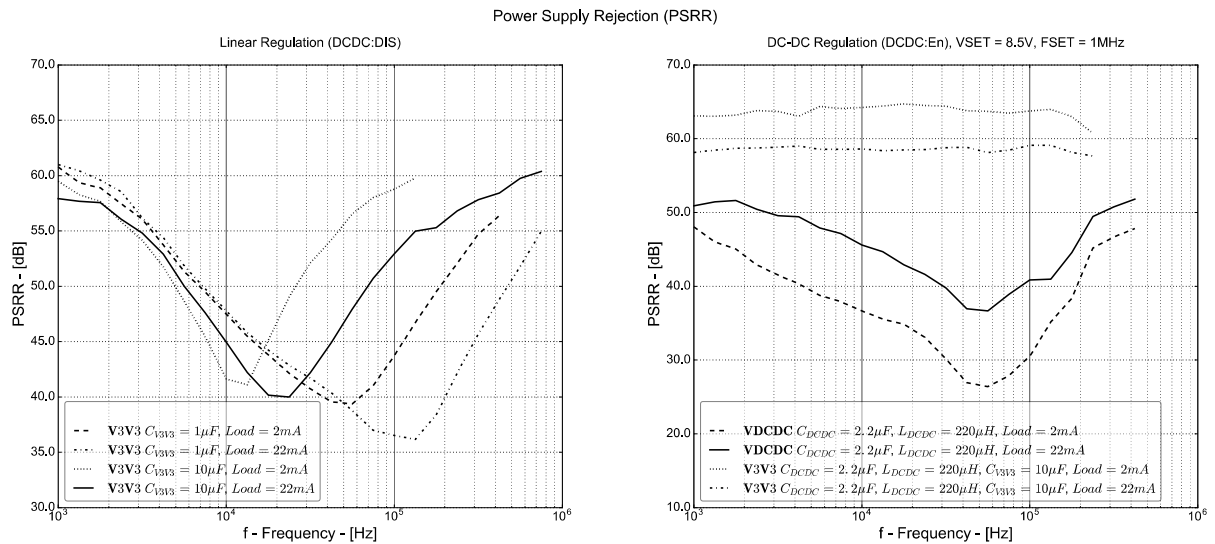
Fig. 19: Power supply rejection ratio under different conditions of C_{V3V3} and I_{V3V3}
