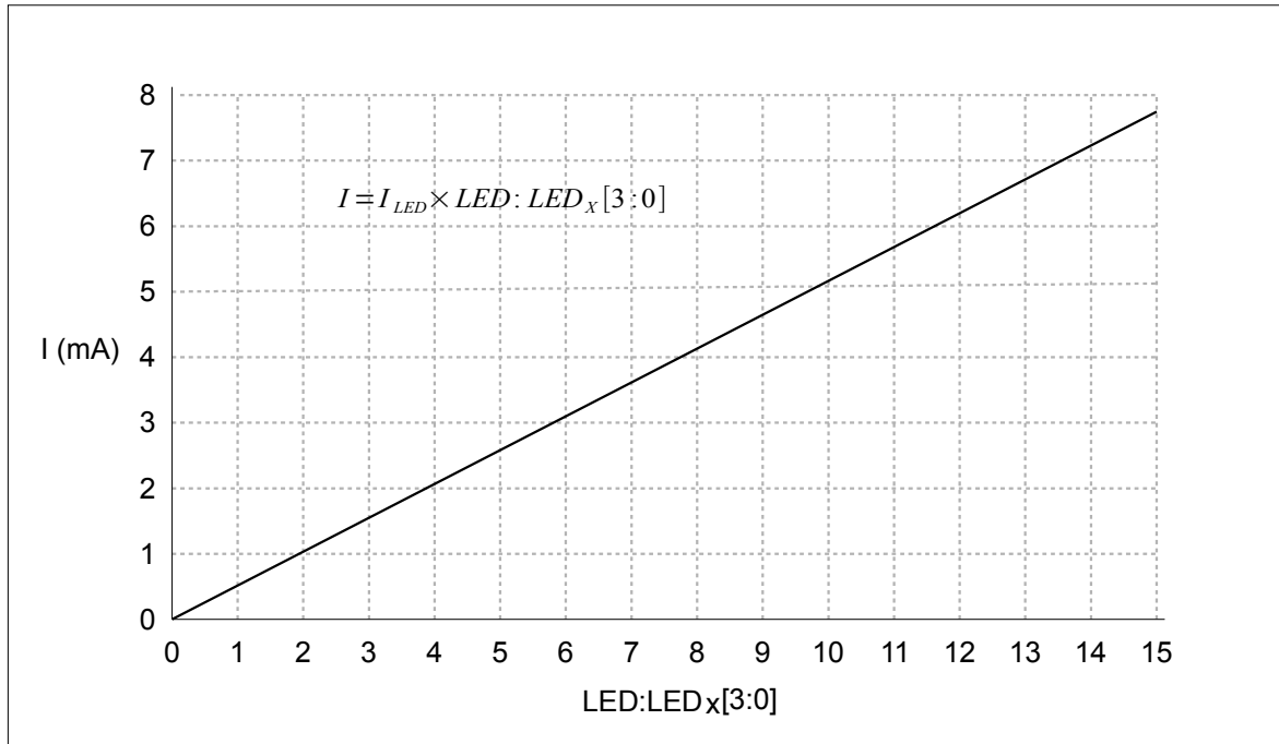
Fig. 13: HMT7748 LED currents
