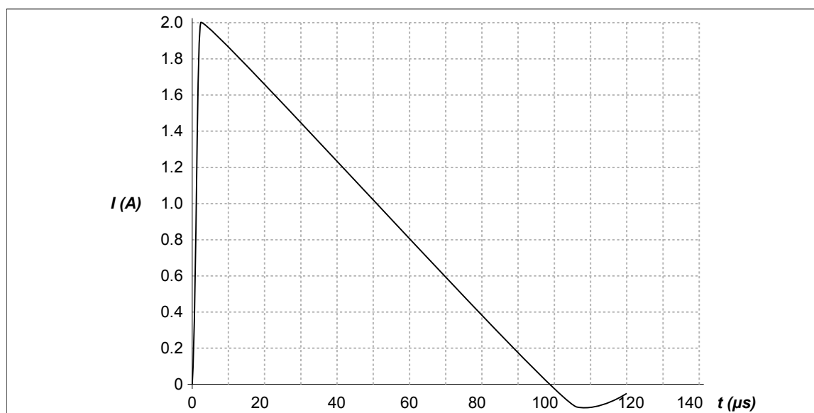
Fig. 20: Surge waveform
