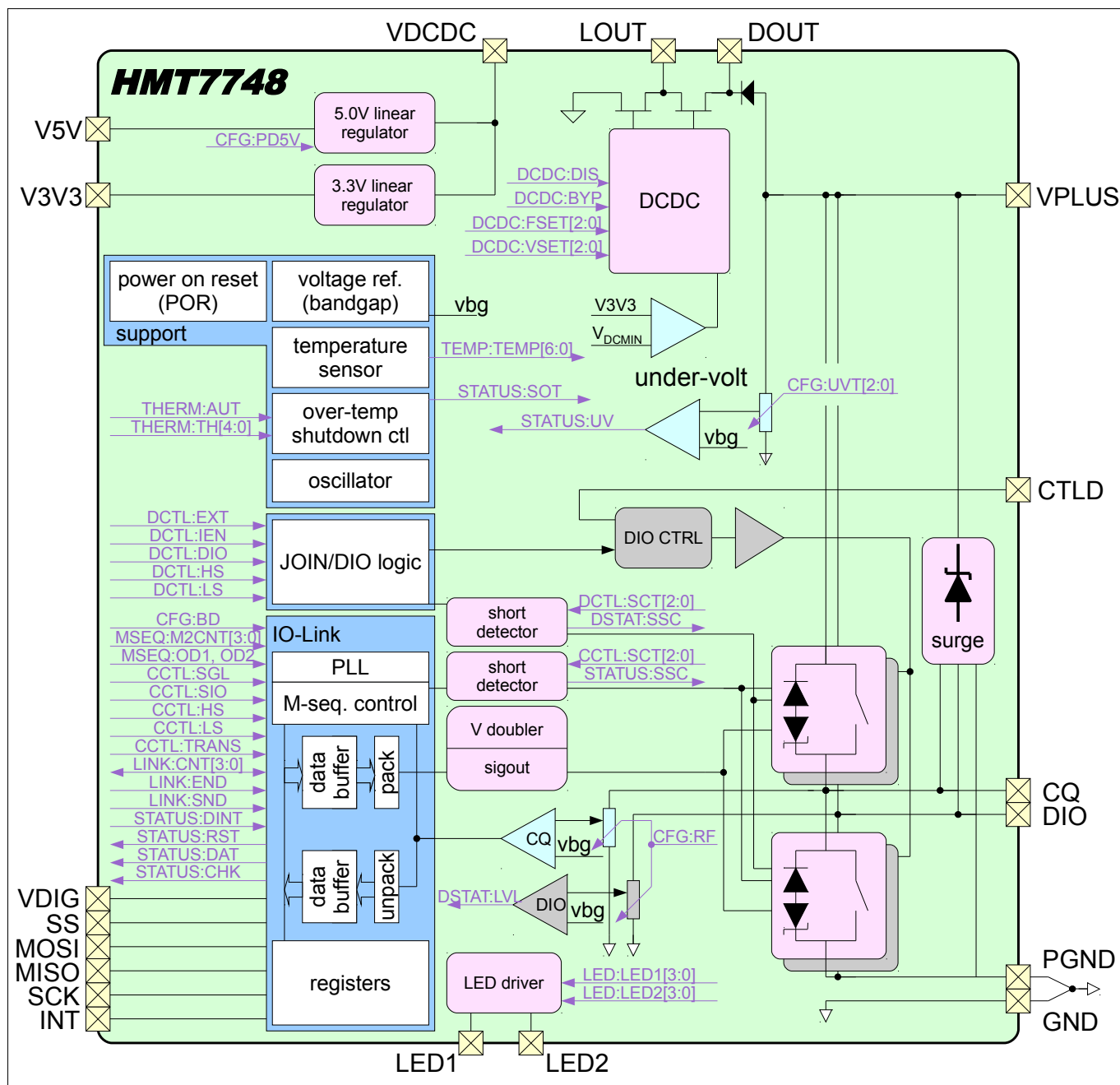
Fig. 21 Detailed block diagram, showing register field connections
