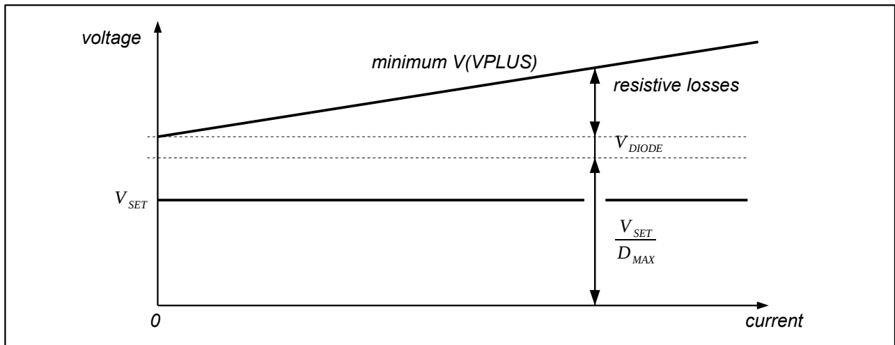
Fig. 15: Minimum supply voltage
