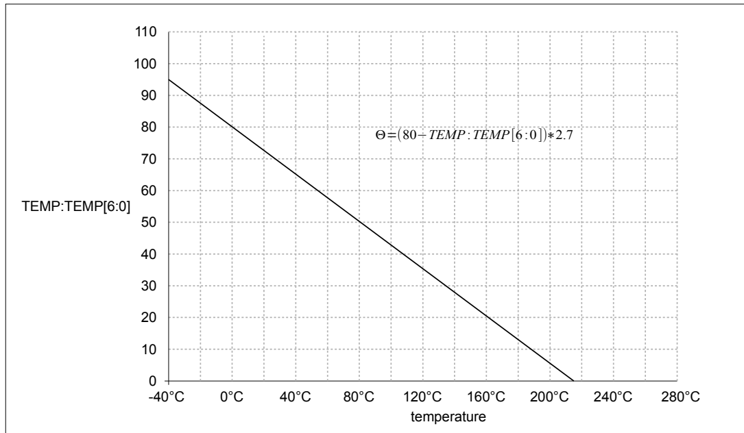
Fig. 11 HMT7748 temperature measurement
