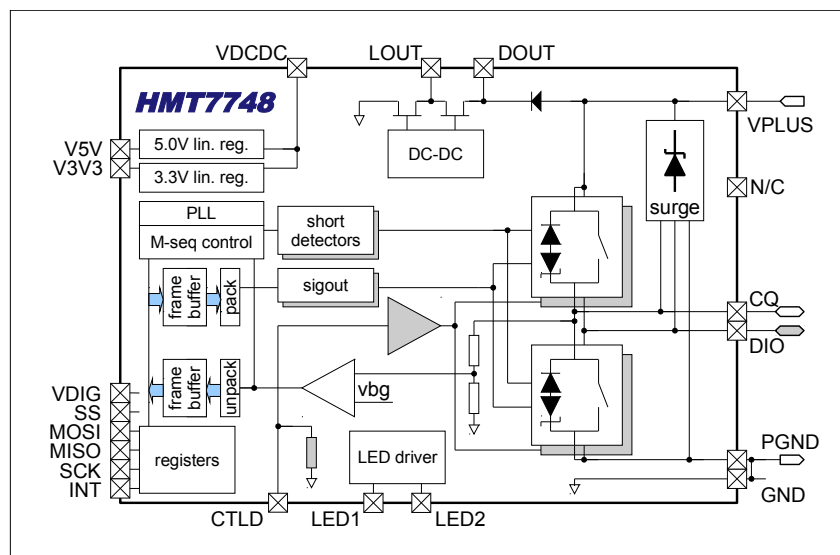
Fig. 1 HMT7748 block diagram. See Fig. 21 for detailed block diagram
