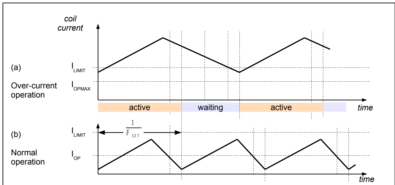
Fig. 16: Over-current operation
