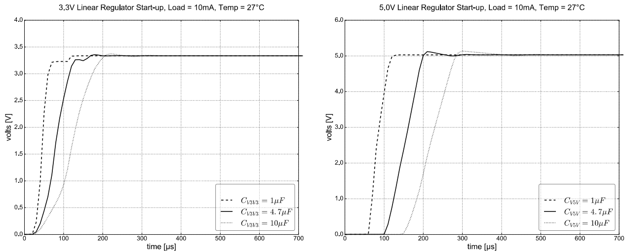
Fig. 17: HMT7748 linear regulators' start-up under different conditions of load capacitance
