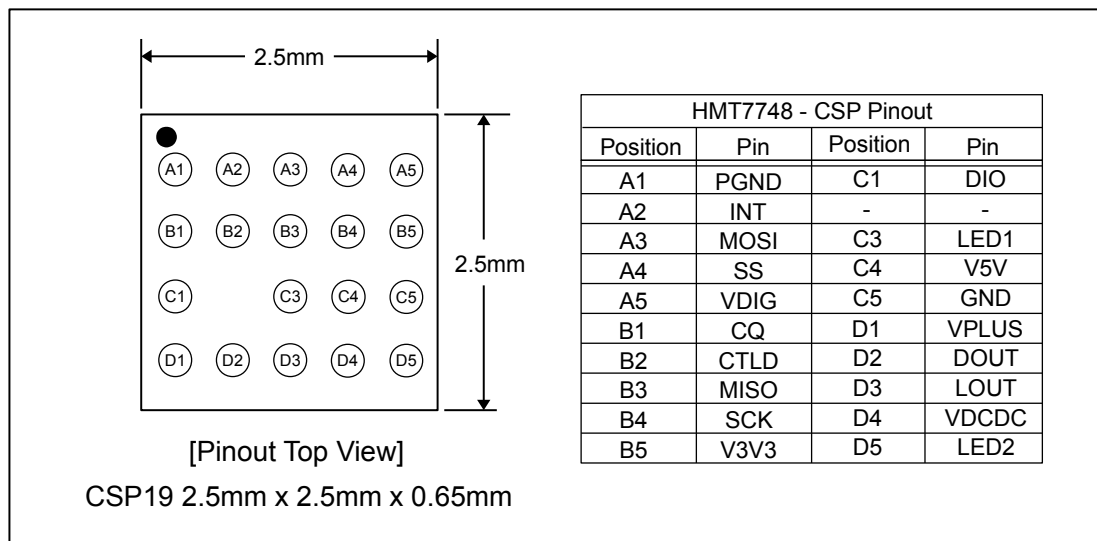
Fig. 3: Package and pinout - CSP
